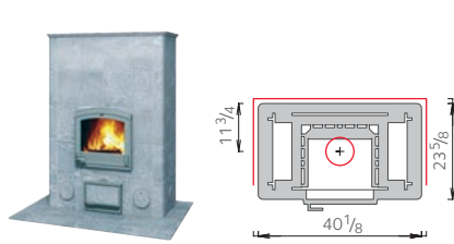
TU2200 • Weight 4056 lbs • Height 60 1/4"
