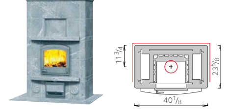
TU2200/5 • Weight 4144 lbs • Height 65"
