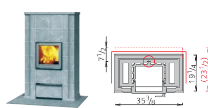
SILO/C • Weight 2755 lbs • Height 60 1/4" SILO/C T • Weight 3174 lbs • Depth 23 1/2"
