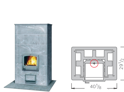
TTU2700/4 • Weight 5688 lbs • Height 72"
