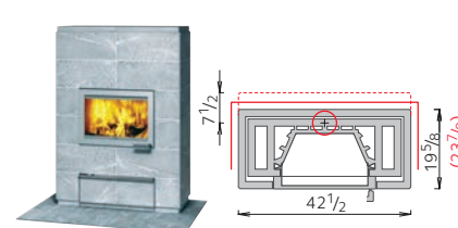
VALKIA • Weight 3350 lbs • Height 60 1/4" VALKIA T • Weight 3825 lbs • Depth 23 7/8"
