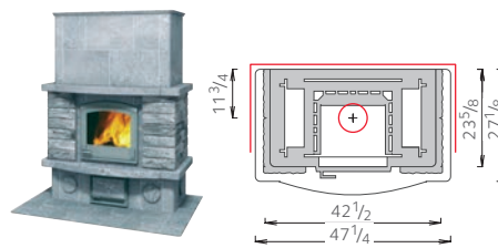
TU2200/1 • Weight 4806 lbs • Height 65"
