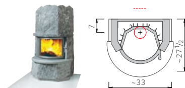
HETTA • Weight ~2138 lbs • Height 60 5/8"
