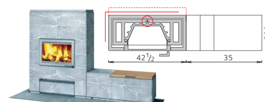
VALKIA + Bench • Weight 3967 lbs • Height 60 1/4" VALKIA T + Bench • Weight 4442 lbs • Depth 23 7/8"
