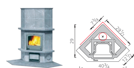
KTU1410/1 • Weight 3042 lbs • Height 65"
