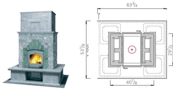
TTU2700/2 • Weight 9612 lbs • Height 86 1/2"
